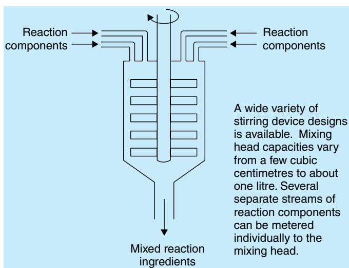
Figure 2.31 Low pressure mixing
